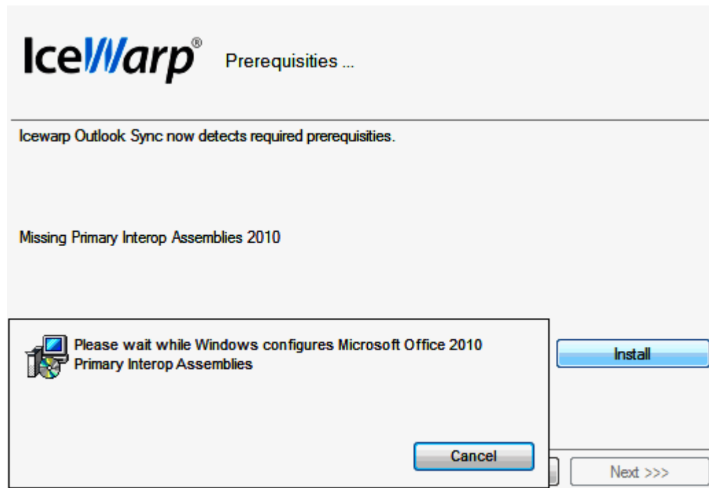
Figure 3 – Prerequisites Page
